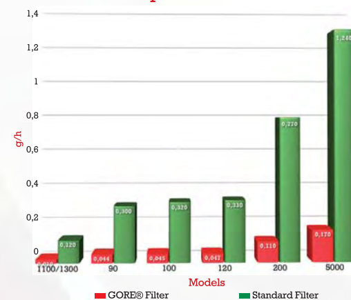
Dulevo Sweepers PM10 Emissions
